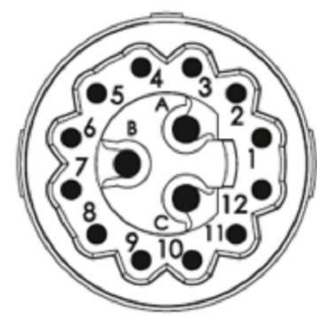
Cable 12+3 Wires
